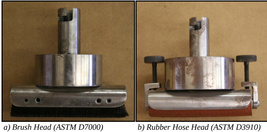
Figure 4.15. Abrasion Heads
