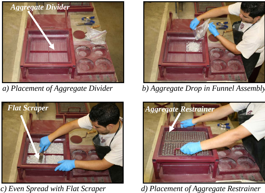
Figure 4.9. Preliminary Aggregate Arrangement
