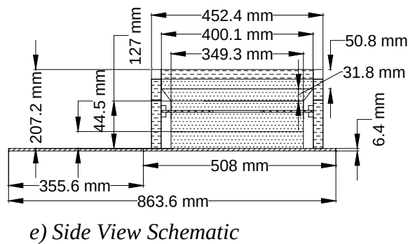
Figure 4.2. Spreader Base
