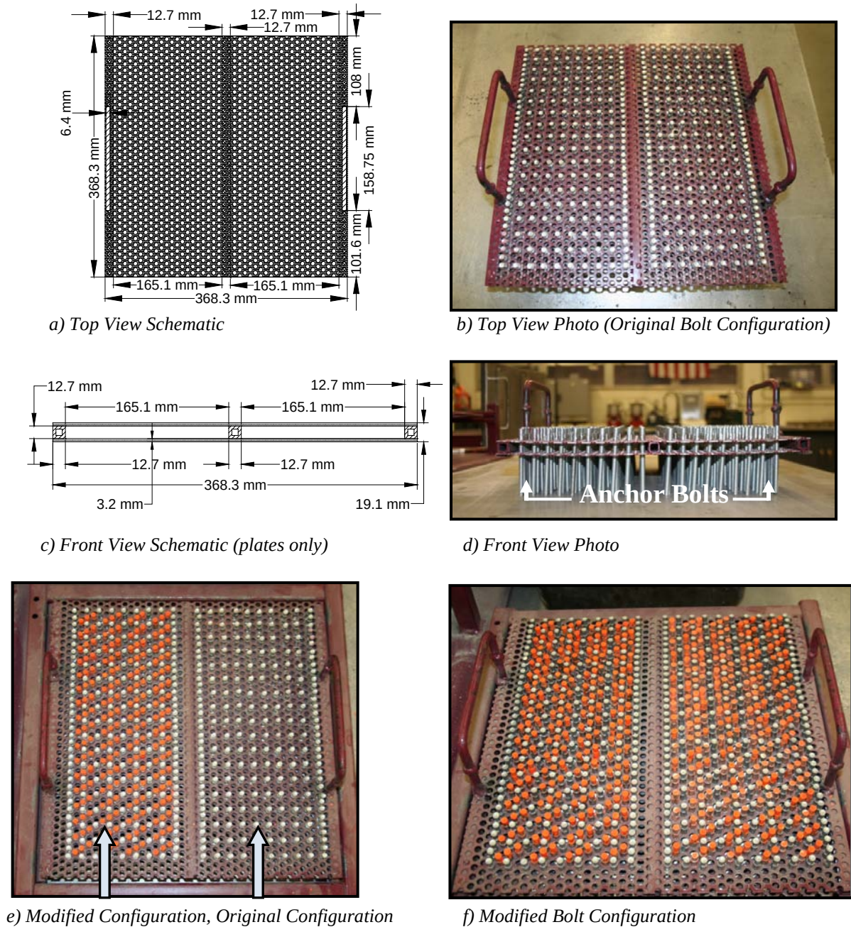
Figure 4.6. Aggregate Restrainer
