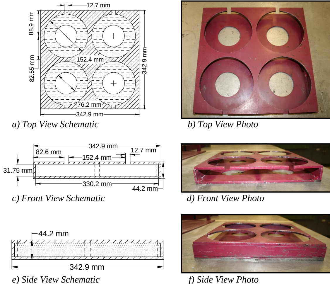
Figure 4.3. Specimen Box
