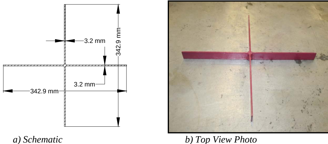
Figure 4.5. Aggregate Divider
