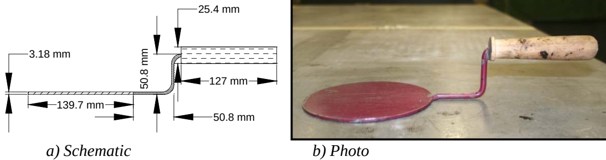
Figure 4.8. Specimen Panhandle
