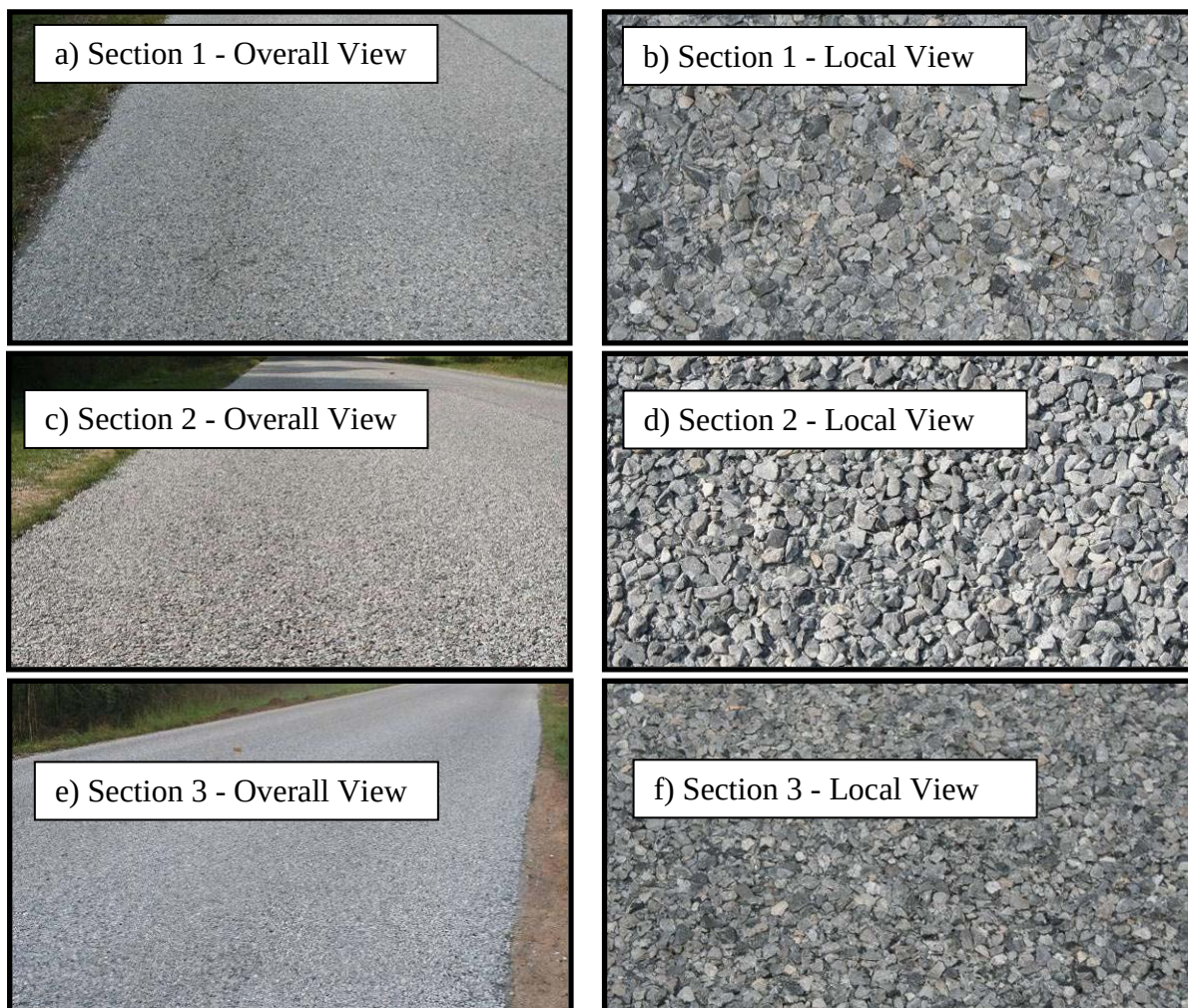
Figure 5.9. Hwy 44 Post-Sealing (09/26/2011)
